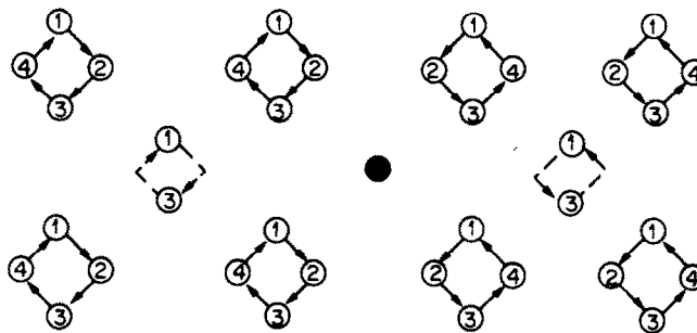
Fig. 3. Stimulus for Demonstration 3. Central fixation spot is shown in black. Left-hand quartet of entraining dots jumped clockwise through four successive positions arranged in a diamond, whilst right-hand quartet was a mirror-image array which jumped counterclockwise. Both the left and right entrained dots, centred within each quartet, actually jumped up and down vertically. However, they were deflected by their immediately surrounding dots along opposite apparent rotary paths (dashed arrows); clockwise for the left dot, counterclockwise for the right dot. See text.
