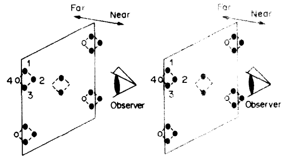
Fig. 4. Deflection of apparent motion in the third dimension. If the reader free-fuses this stereoscopic diagram by diverging his eyes he will see what the stimulus was for Demonstration 4. The four spots in the surround described rotary trajectories in stereoscopic depth. They lay in the fixation plane in frame 1, then jumped downwards and forwards (nearer to the observer) in frame 2, then jumped downwards and backwards (into the fixation plane again) in frame 3, then up and behind the fixation plane in frame 4. The central test spot was seen to perform a similar motion in depth although it was visible only in frames 1 and 3, when it actually lay in the plane of fixation.
