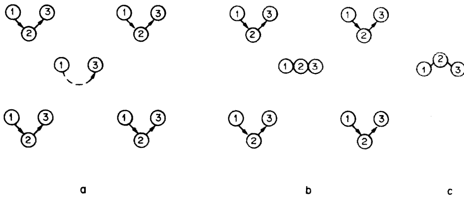
Fig. 1. (a) Path deflection illusion. A square matrix of five spots was presented in frame 1, followed by the same pattern shifted down and to the right in frame 2, and then shifted up and to the right in frame 3. The central spot was deleted from frame 2 so that it appeared only in frames 1 and 3. Numbers in spots show order of presentation. Drawing is not to scale: actual dots were tiny (4 min arc) points of light, not disks. The four spots in the surround were correctly seen as jumping along V-shaped trajectories. The central unpaired spot also appeared to follow a V-shaped trajectory (dashed arrow), even though it had no partner to pair with in frame 2. If the four surround dots were removed (not shown), the central spot was correctly seen as oscillating horizontally instead of describing a V. (b) Motion contrast illusion. Display was the same as a except that the central dot was visible in frames 1, 2 and 3, jumping along a straight line. Result: the central dot appeared to move along a slight upward V, as shown diagrammatically in (c).
