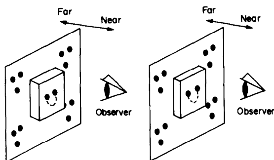
Fig. 5. Disparity-specific motion entrainment. If the reader free-fuses this stereoscopic diagram by diverging his eyes he will see what the stimulus was for Demonstration 5. All the dots moved in frontoparallel planes but the central dot lay in a different depth plane in front of the four entraining dots. Motion entrainment was weaker but still visible.
