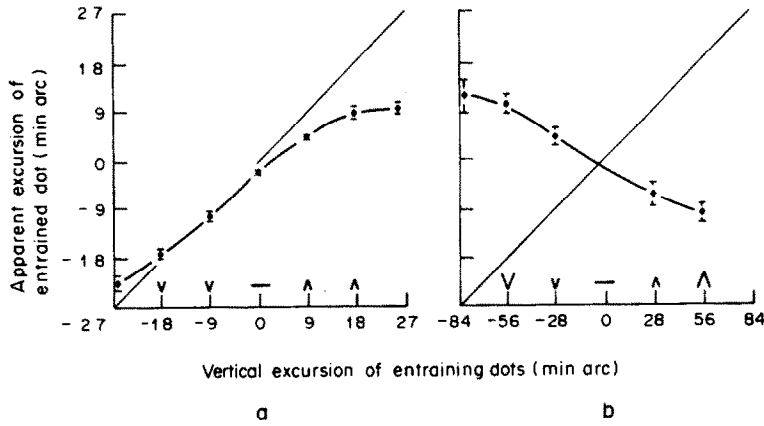
Fig. 2. (a) Path deflection in of the central dot in Experiment 1 [Fig. 1(a)] as a function of the amplitude of the V-shaped trajectories of the four spots in the surround. Each datum point is the mean of 30 readings (3 subjects \times 10 readings). Vertical bars show standard errors of the 30 pooled readings. Apparent deflections entrained into the central dot were about half the actual vertical deflections of the surround dots. (b) Motion contrast induced into the central dot in Experiment 2 [Fig. 1(b)]. Each datum point is the mean of 6 readings (2 subjects \times 3 readings). Apparent deflection of central dot was now opposite to the actual vertical deflection of surround dots. Slope of best fitting line was -0.177 . Note that (a) and (b) have different abscissae.
