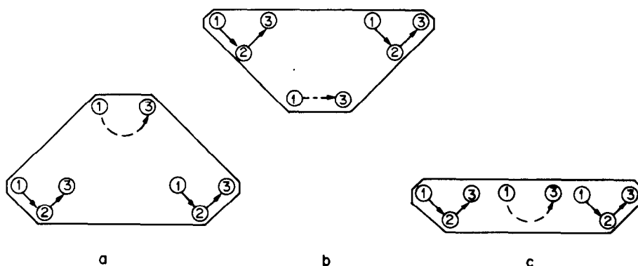
Fig. 6. Entraining dots can pull (a, c) but not push (b) a deflection into a dot's path. Dashed arrows show apparent path of the central dot, which shows entrainment in a and c but not in b. Thin line around dots is the convex envelope outside which, we conjecture, motion cannot be entrained.
